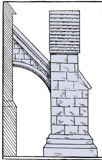
FLYING BUTTRESS
